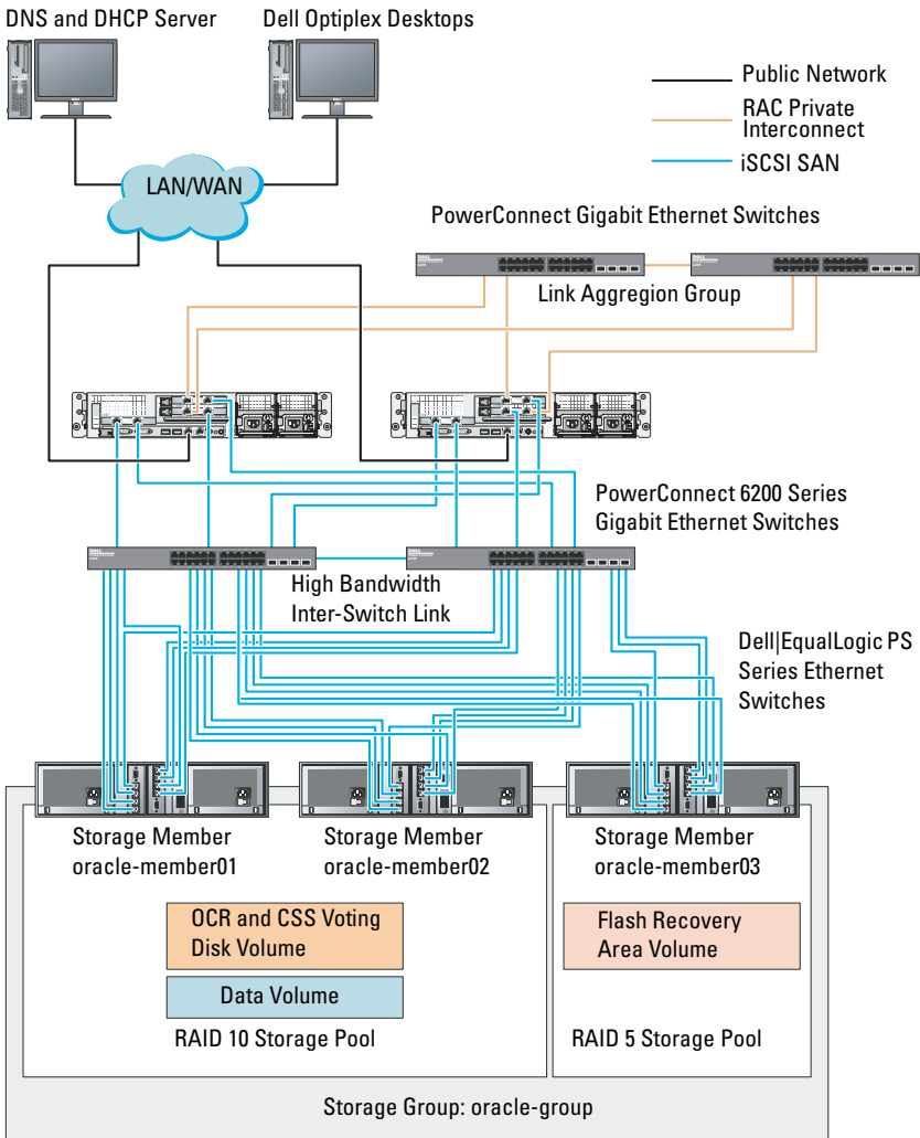
Figure 6-2. Configuring a Sample Oracle RAC With Three PS6000XV Arrays
